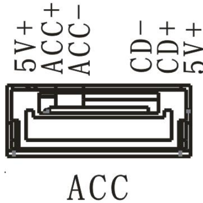
ACC连接器示意图 Schematic Diagram of the ACC Connector
