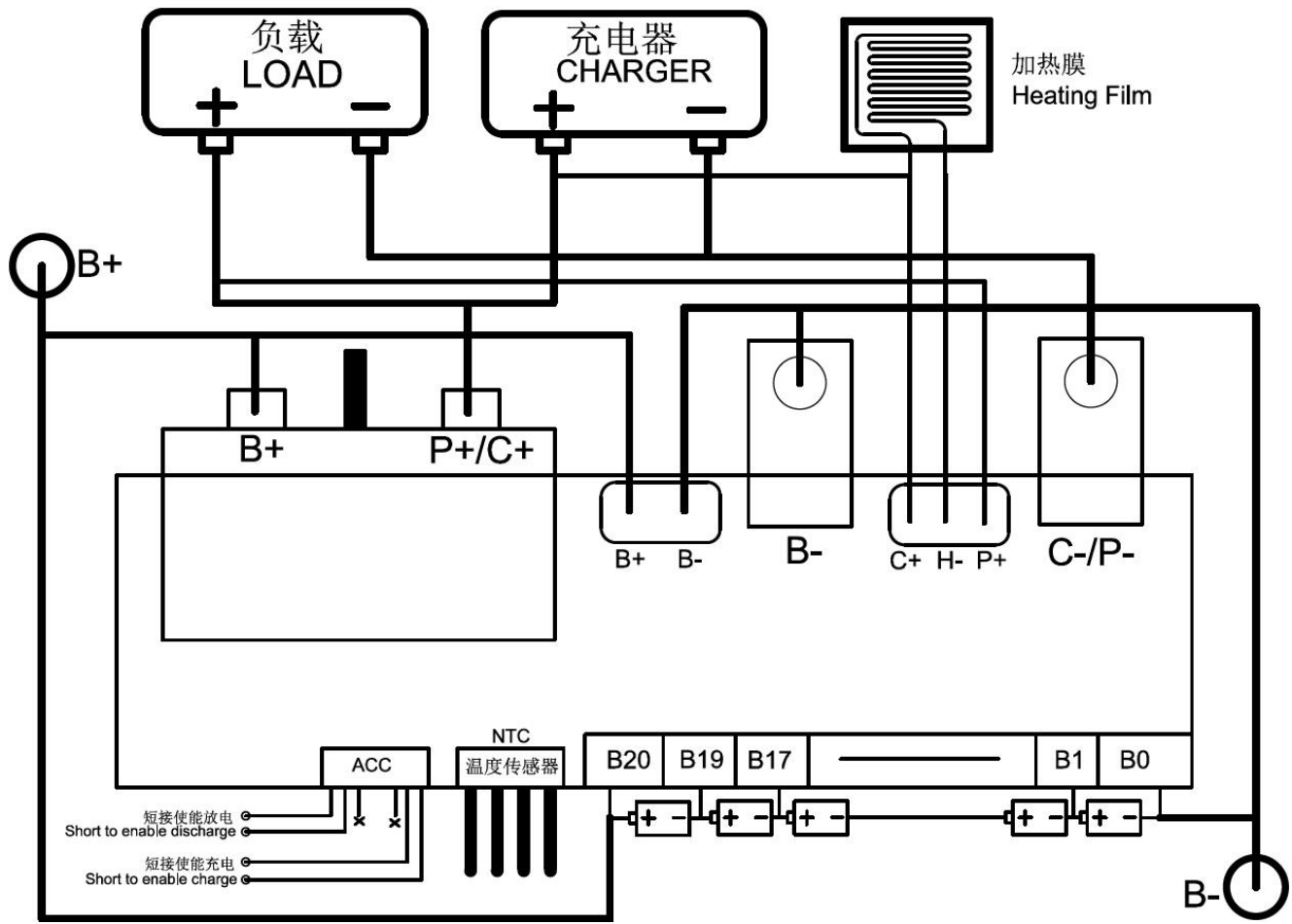
JK-B2A20S-CR60P接线图 JK-B2A20S-CR60P wiring diagram
