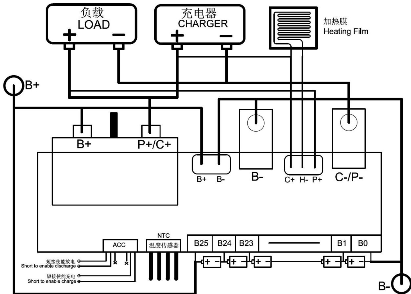
JK-B2A25S-CR60P接线图 JK-B2A25S-CR60P wiring diagram
