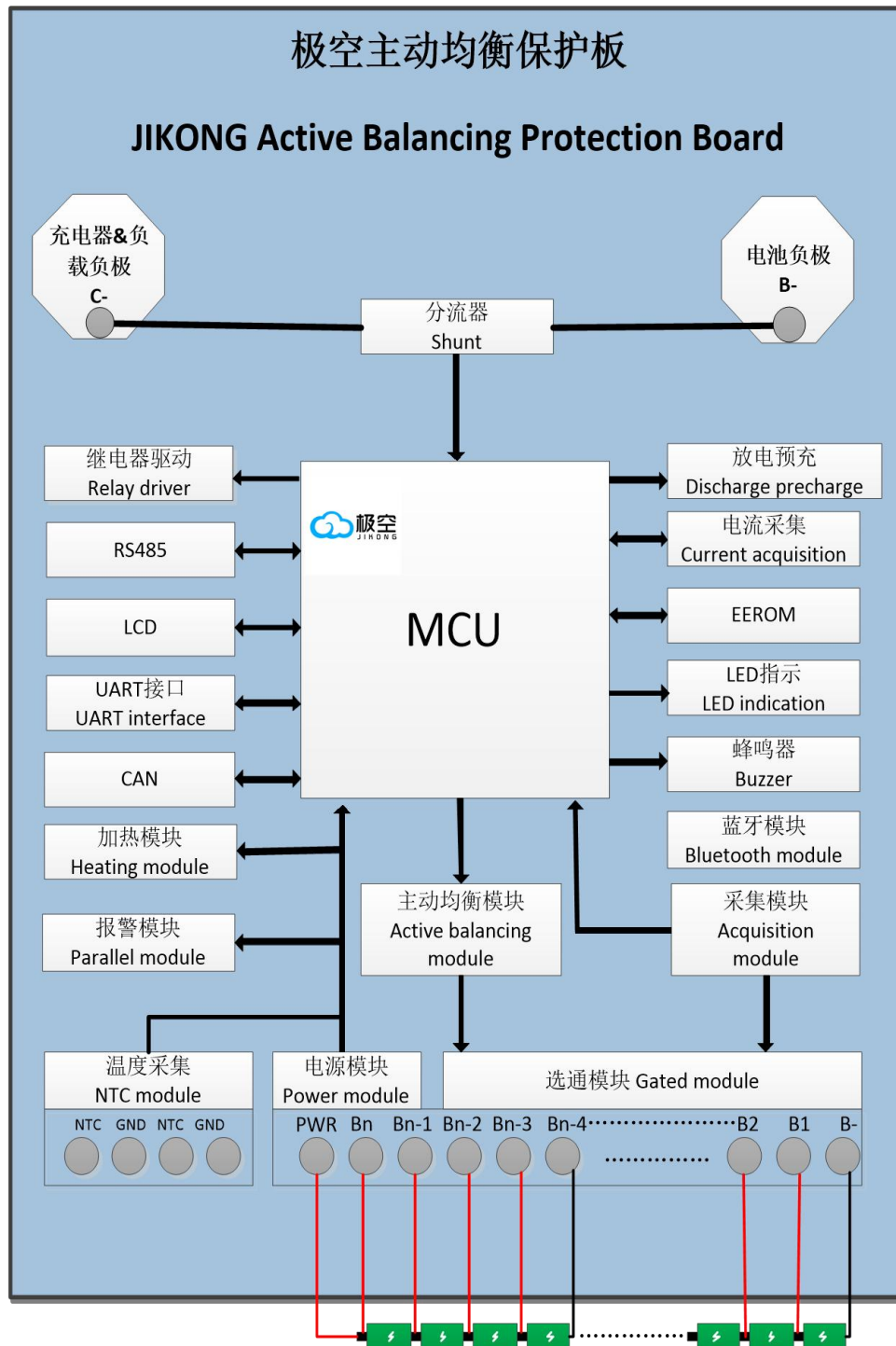
JK-B2A25S-CR60P 结构框图 JK-B2A25S-CR60P structure block diagram
