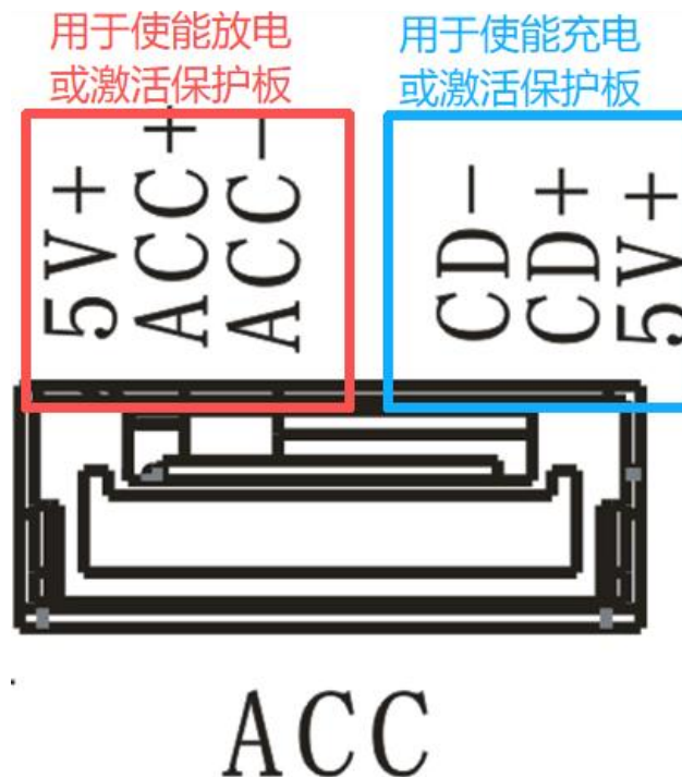
ACC接口示意图 Schematic Diagram of the ACC Interface
