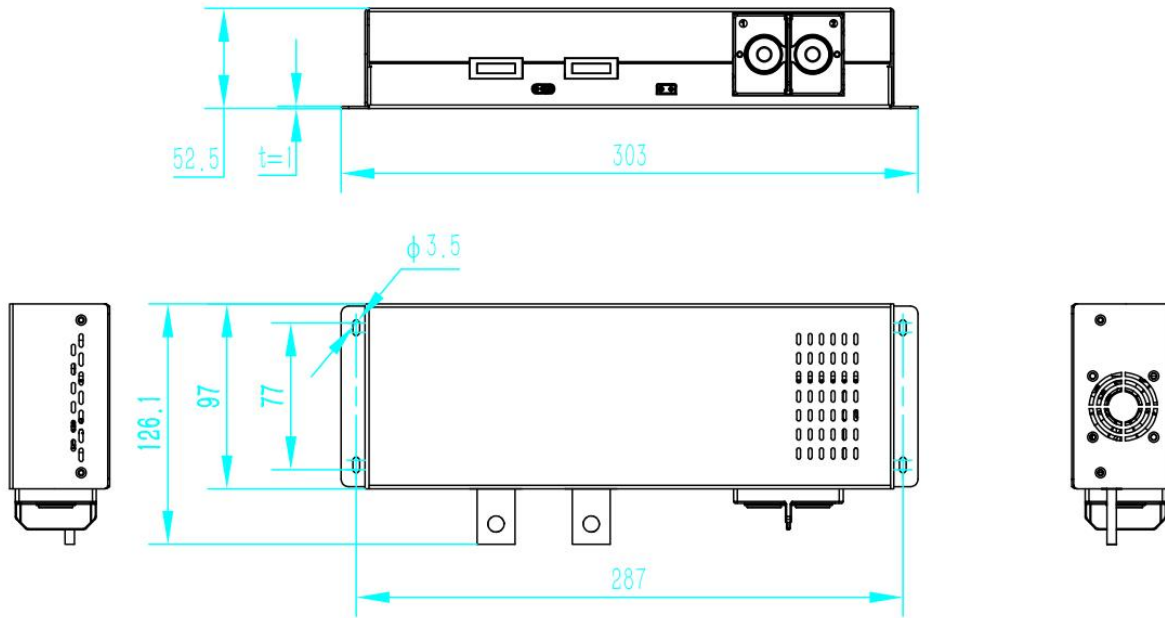
JK-B2A25S-CR60P 外形尺寸 Dimensions of JK-B2A25S-CR60P
